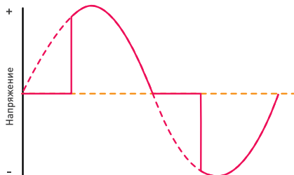
Forward-phase (TRIAC)
